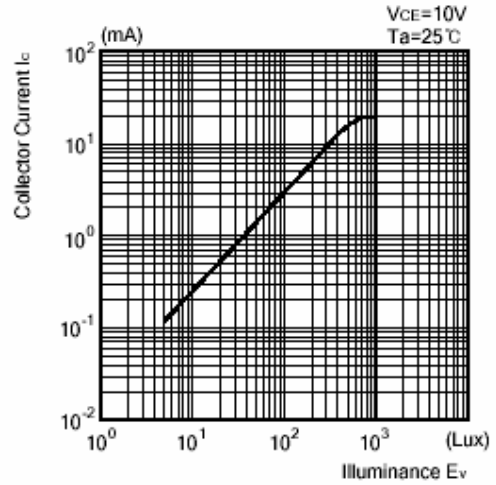
● Collector Current / Illuminance I_c/E_v
