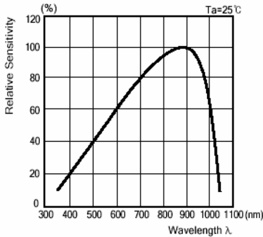
● Spectral Sensitivity
