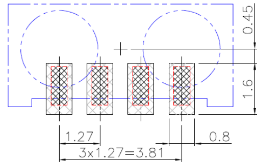
Example of Mounting drawing from Solder Side (Reference)
