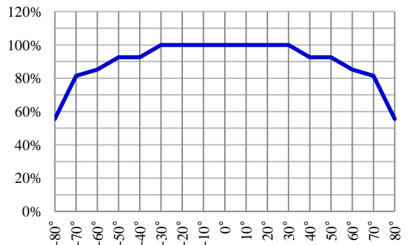
[ Fig.7 ] Directivity
